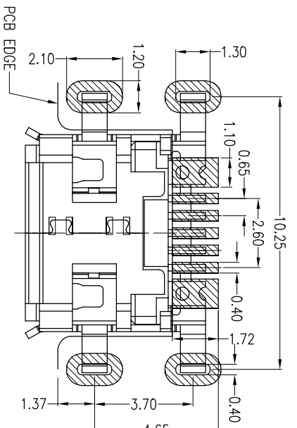
RECOMMENDED PCB LAYOUT PCB图仅供参考
