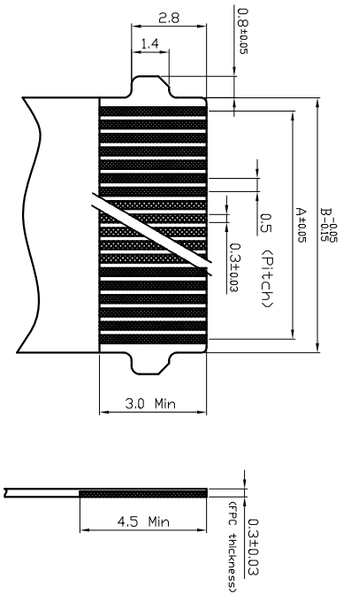
适用FPC寸法(带勾) APPLICABLE FPC(+LOCK)
