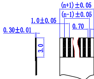
FFC/FPC Dimension
