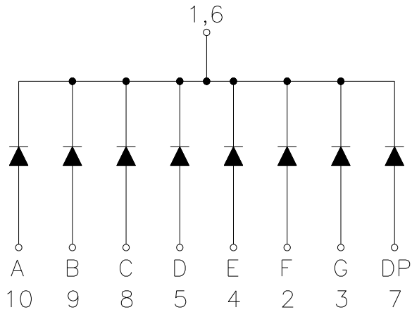
Common Cathode
