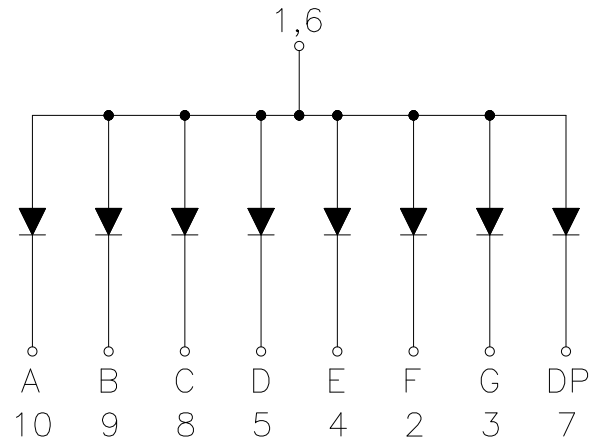
Common Anode
