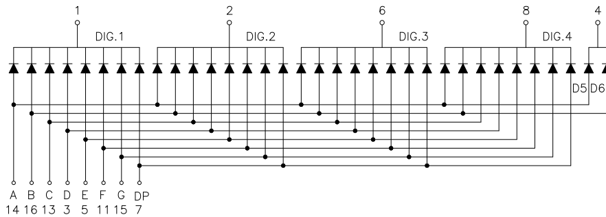
Common Cathode
