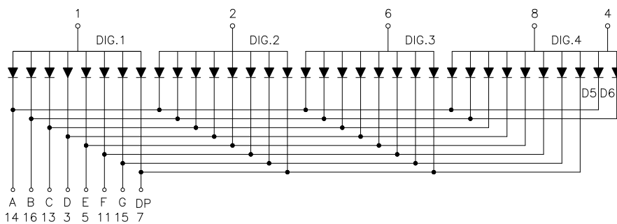
Common Anode
