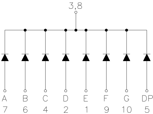
Common Cathode
