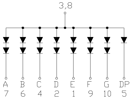
Common Anode
