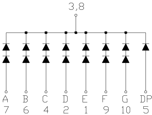
Common Cathode
