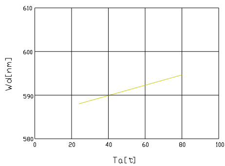
Fig.5-Dominant Wavelength(@250mA) vs. Ambient Temperature
