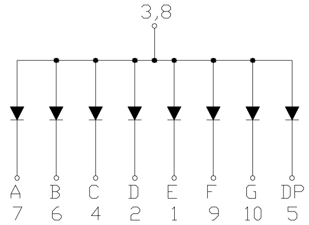
Common Anode
