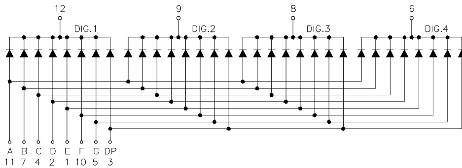
Common Cathode
