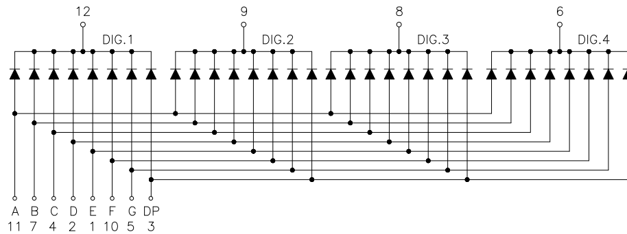
Common Cathode
