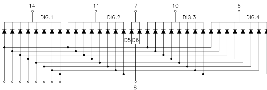
Common Cathode
