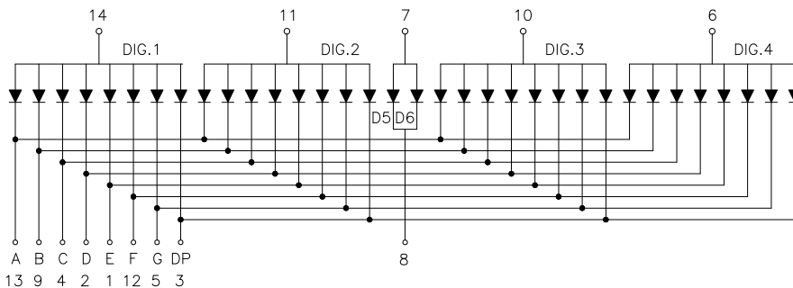
Common Anode
