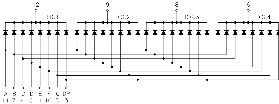
Common Cathode
