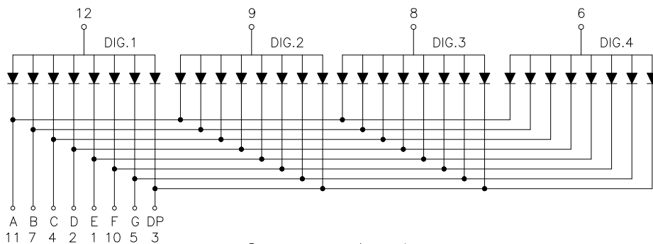
Common Anode
