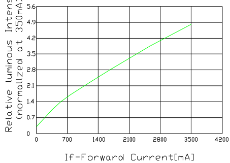
Fig.1-Relative luminous Intensity vs. Forward Current
