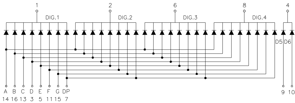
Common Cathode
