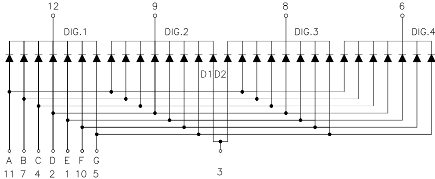
Common Cathode
