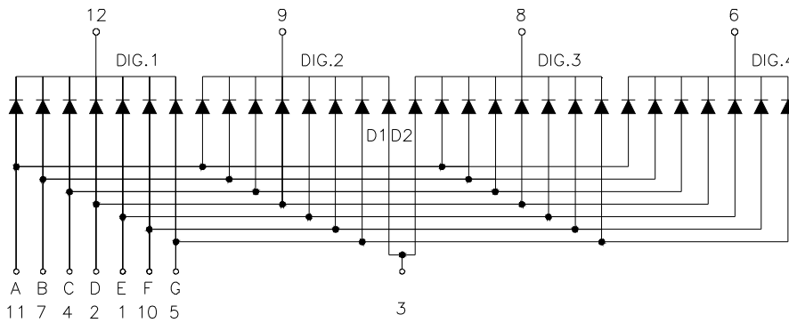
Common Cathode
