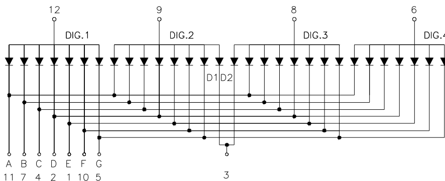
Common Anode
