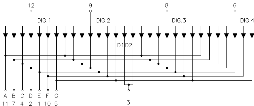
Common Anode
