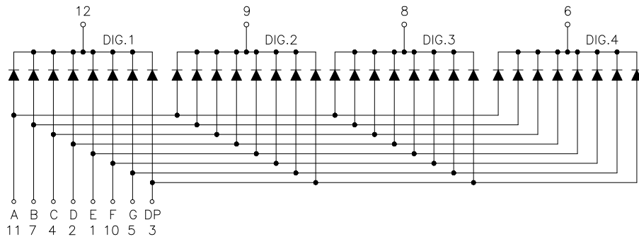
Common Cathode
