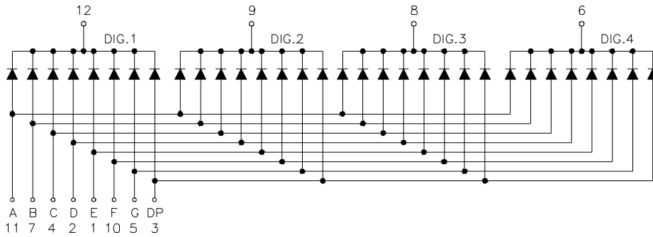
Common Cathode
