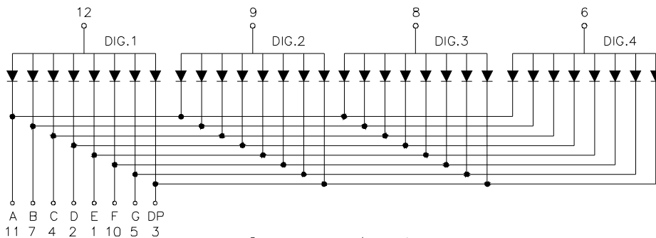
Common Anode
