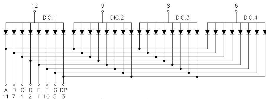
Common Anode
