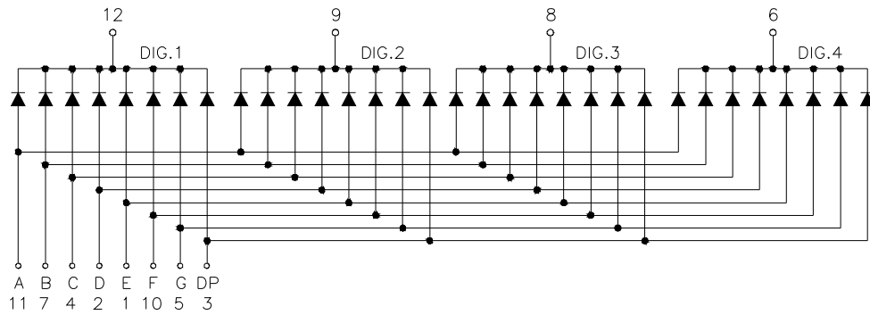
Common Cathode
