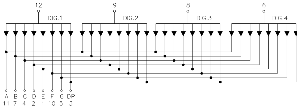
Common Anode
