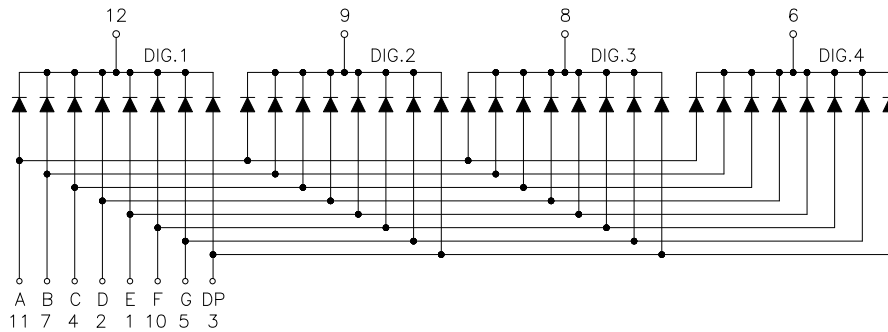
Common Cathode
