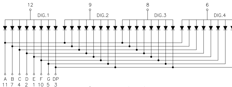
Common Anode
