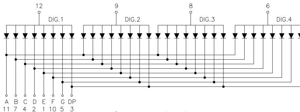
Common Anode
