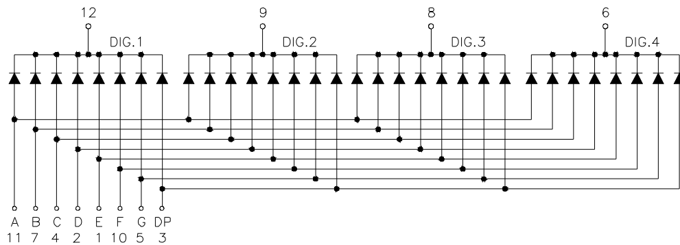
Common Cathode
