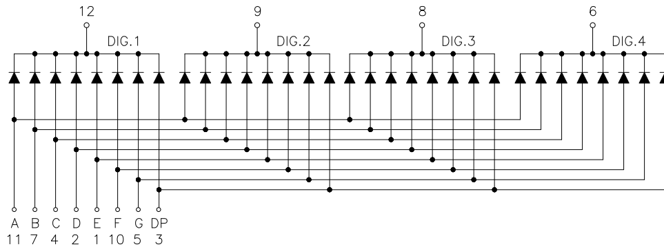
Common Cathode
