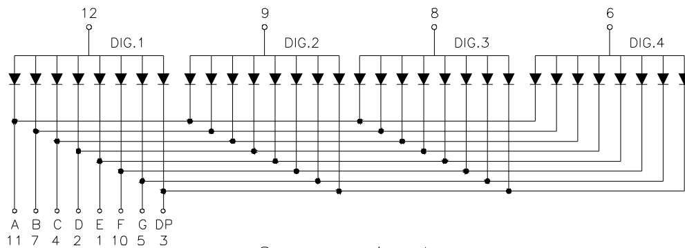
Common Anode
