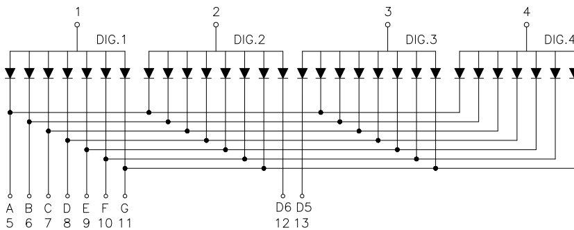
Common Anode
