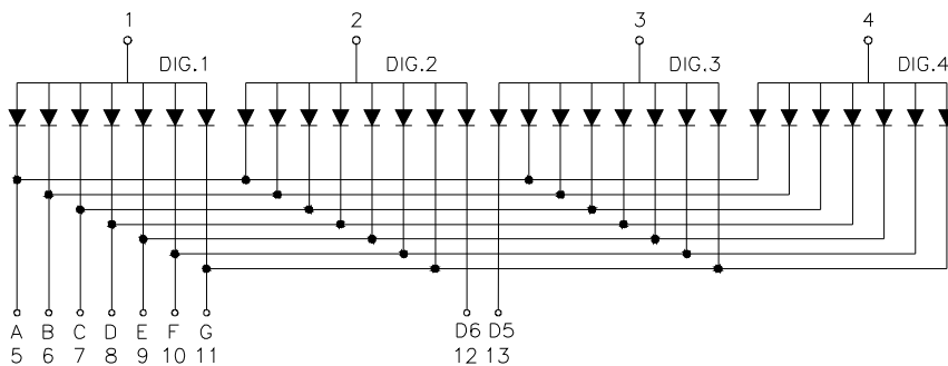
Common Anode
