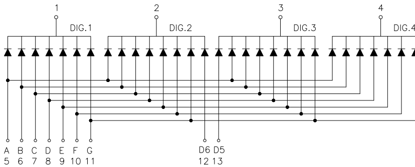
Common Cathode
