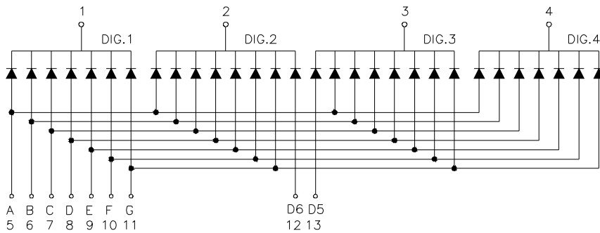
Common Cathode
