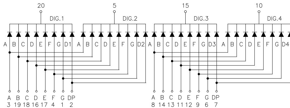
Common Cathode
