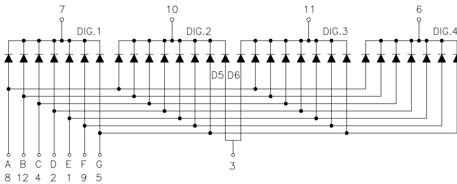
Common Cathode
