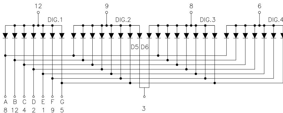
Common Anode
