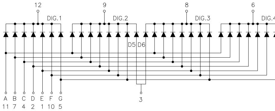
Common Cathode
