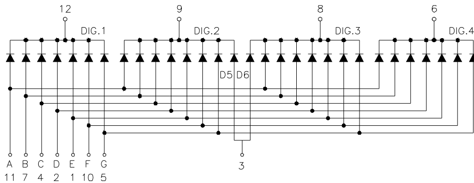
Common Cathode
