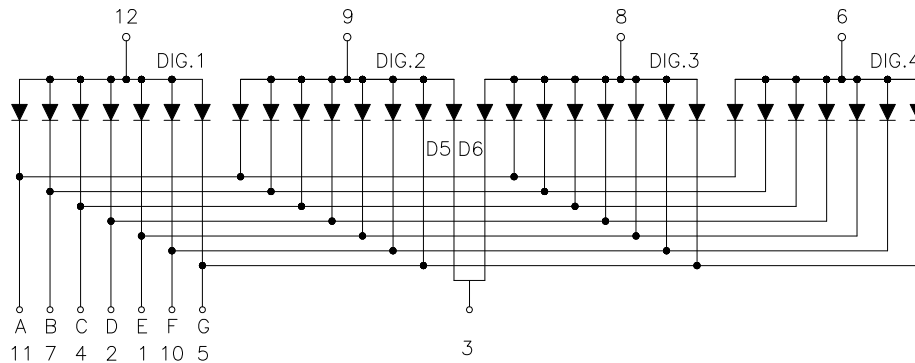
Common Anode
