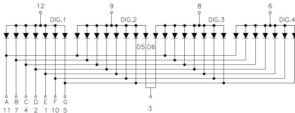
Common Anode
