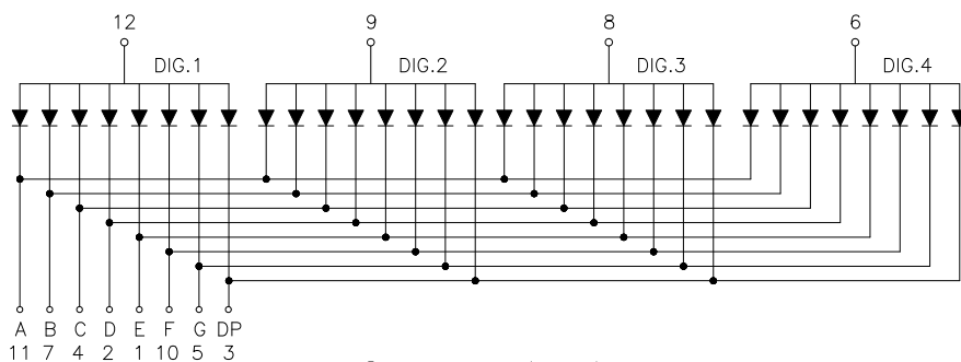
Common Anode
