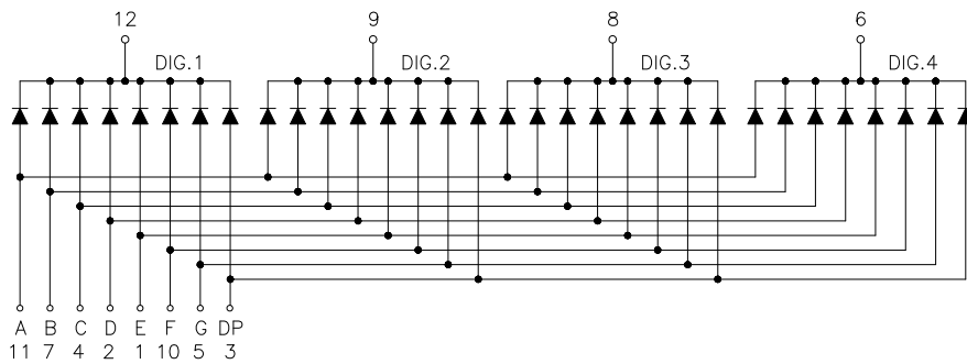
Common Cathode
