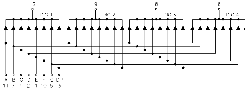
Common Cathode
