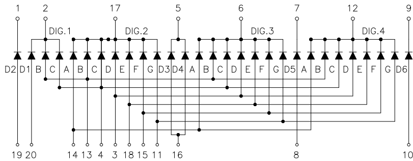
Common Cathode
