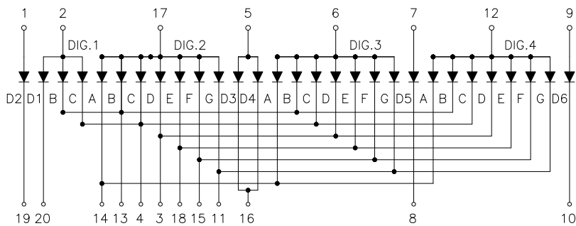
Common Anode
