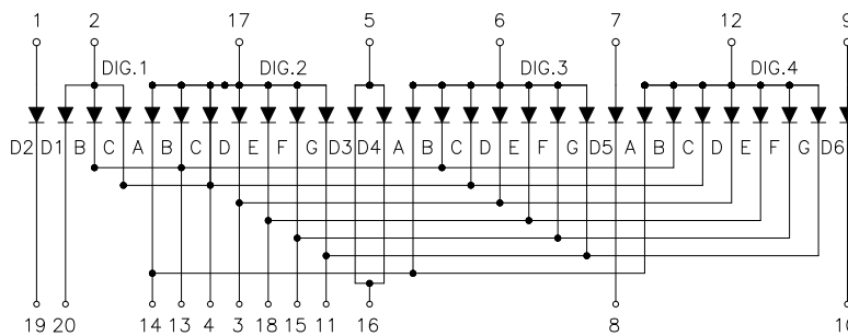
Common Anode
