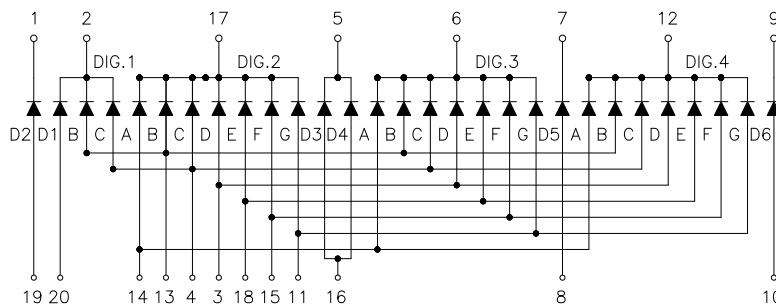
Common Cathode
