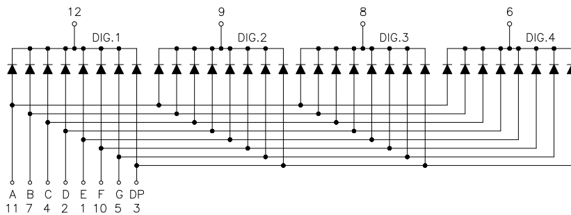
Common Cathode
