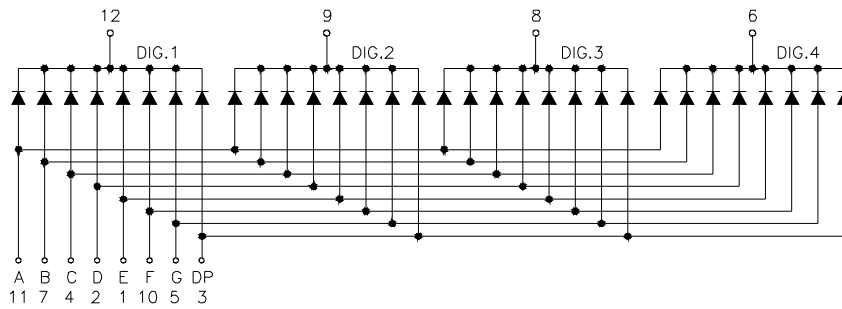
Common Cathode
