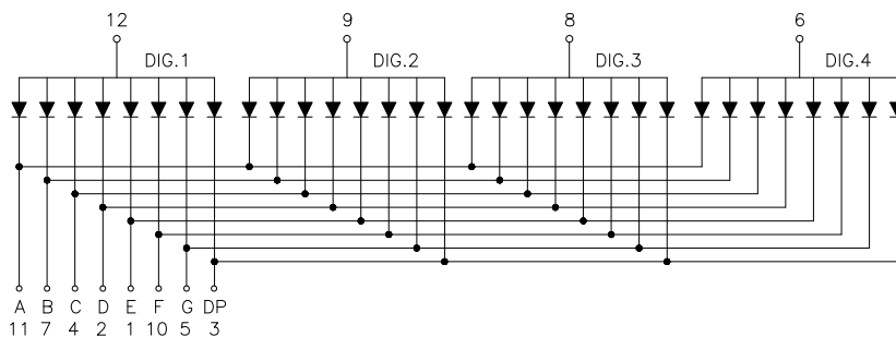
Common Anode
