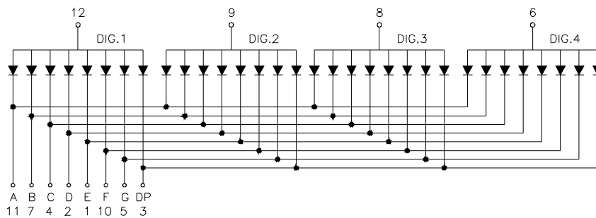
Common Anode
