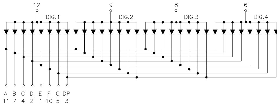
Common Anode
