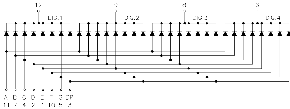
Common Cathode
