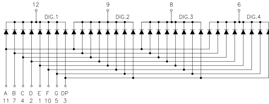
Common Cathode
