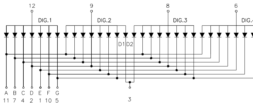
Common Anode
