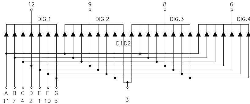
Common Cathode
