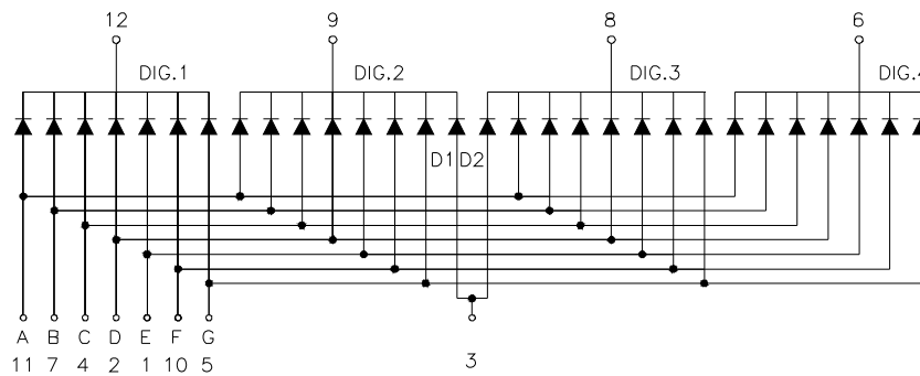
Common Cathode
