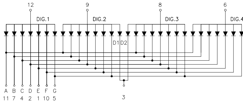
Common Anode
