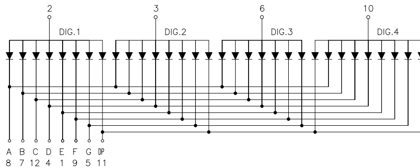
Common Anode
