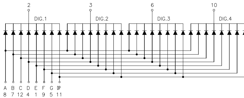
Common Cathode
