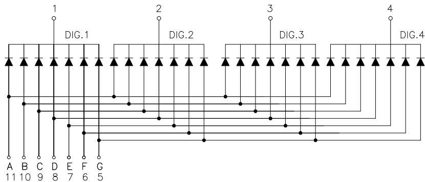
Common Cathode
