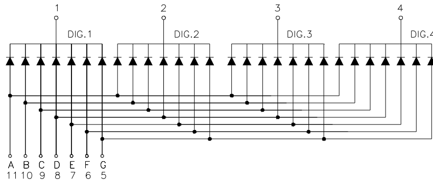
Common Cathode
