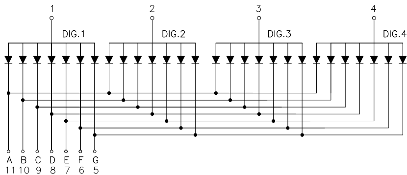
Common Anode
