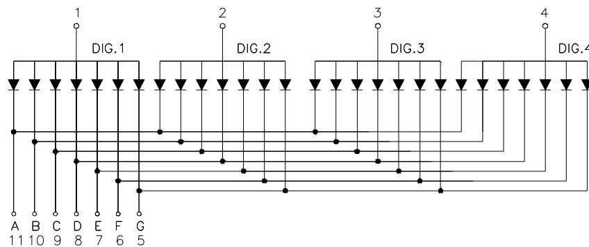
Common Anode
