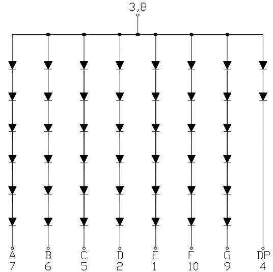
Common Anode
