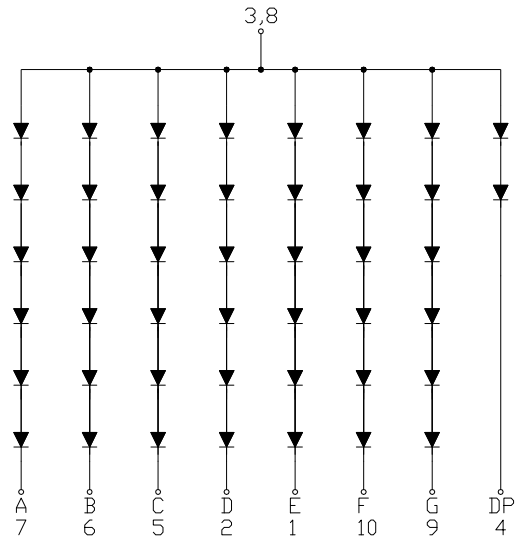
Common Anode
