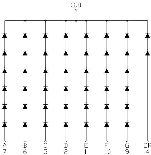
Common Cathode
