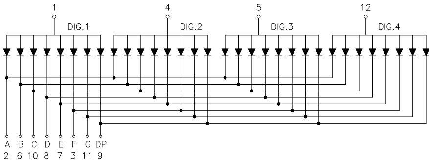
Common Anode
