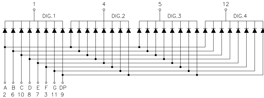
Common Cathode
