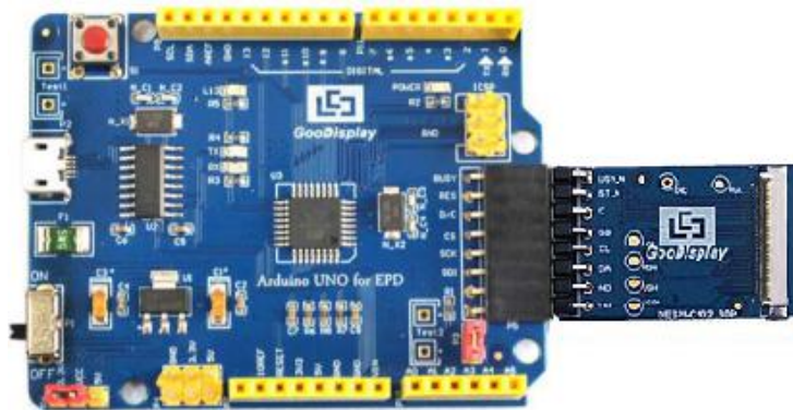
Figure 3 : Connection between DESPI-C102_30P and motherboard
