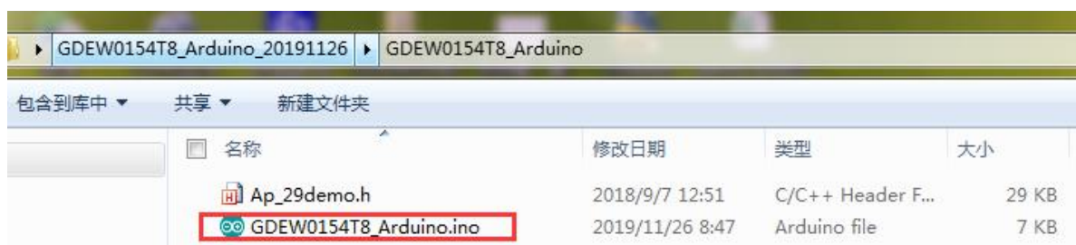
Figure 5 : Open Arduino.ino
